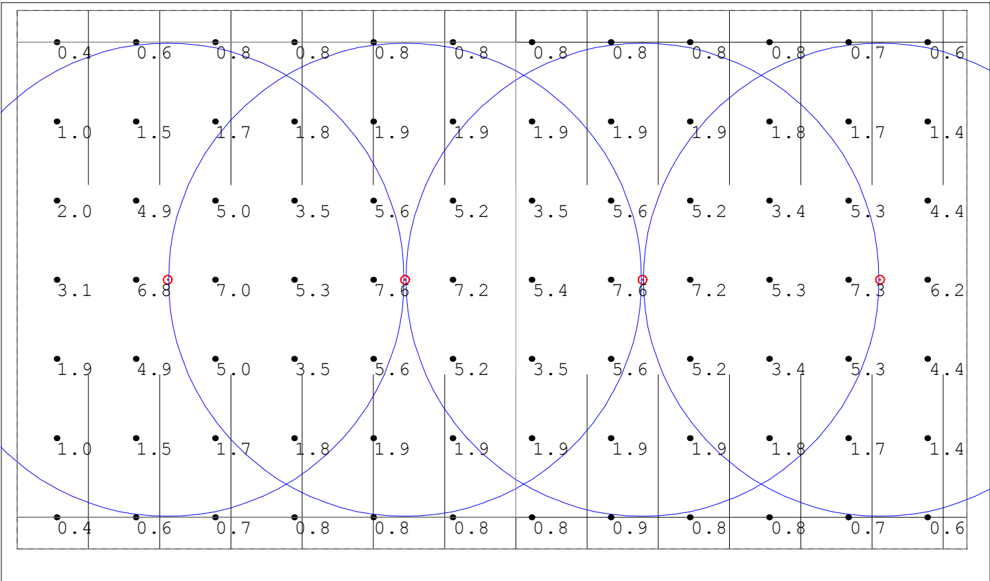
Fixtures surface mounted at 10' | 10' x 10' calculation grid at surface
